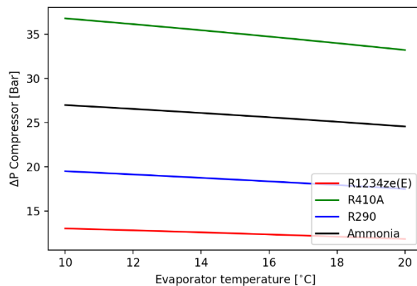
Figure 7. Compressor pressure difference (Tcond=70°C)
