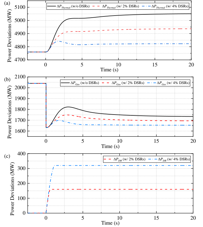
Fig. 5 Power deviations in the three cases: (a) the total power deviations of the reheat steam generators, (b) the total power deviations of the gas turbine generators, (c) the regulation power provided by DSRs.
