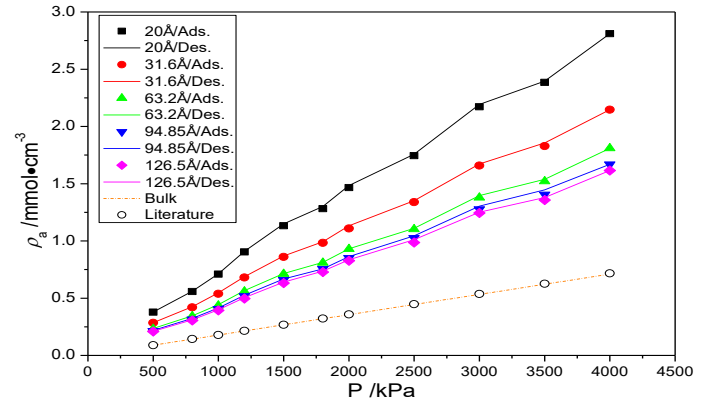
Fig 2 Simulated adsorption isotherms of CO 2 in 'L' shaped carbon slit pores at 673.15 K
