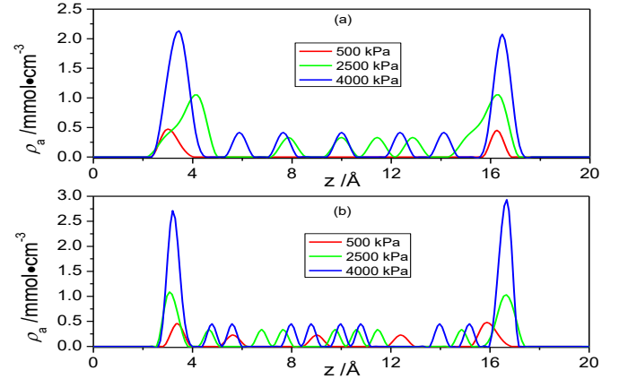
Fig 9 1D local CO 2 density profile along z direction in slit pore a and b of 'L' shaped carbon slit pore of height 20Å at 873.15 K. (a) and (b) represents density profile in section 'a' and 'b' of 'L' shaped carbon slit pore respectively.
