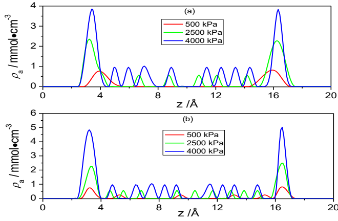
Fig 8 1D local CO 2 density profile along z direction in slit pore a and b of 'L' shaped carbon slit pore of height 20Å at 673.15 K. (a) and (b) represents density profile in section 'a' and 'b' of 'L' shaped carbon slit pore respectively.
