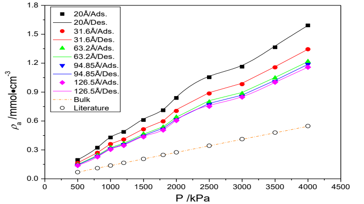
Fig 3 Simulated adsorption isotherms of CO 2 in 'L' shaped carbon slit pores at 873.15 K
