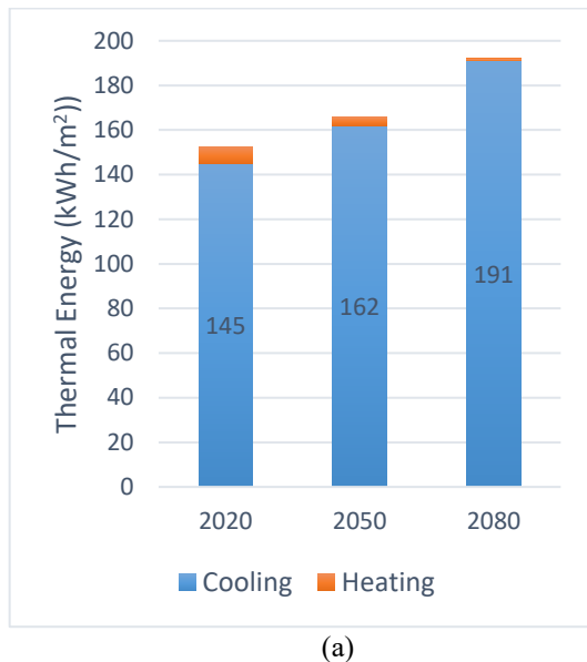
Fig.2. Thermal energy demand for cooling and heating (a) annual; (b) hourly peak
