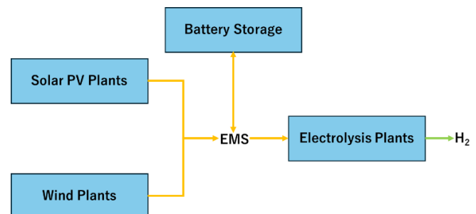
Fig. 1 Proposed energy system for green H 2 production
