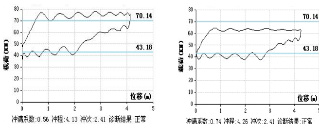
Figure 2. Work diagram of well 1# before and after injection
