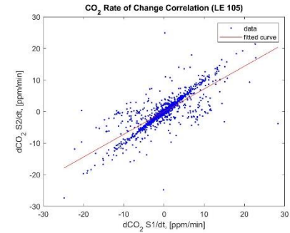
Fig. 11. CO 2 change in concentration correlation for sensor S1 and S2 in LE 105
