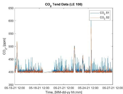
Fig. 6. CO 2 concentration readings for LE 100
