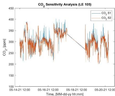
Fig. 9. CO 2 concentration readings for LE 105
