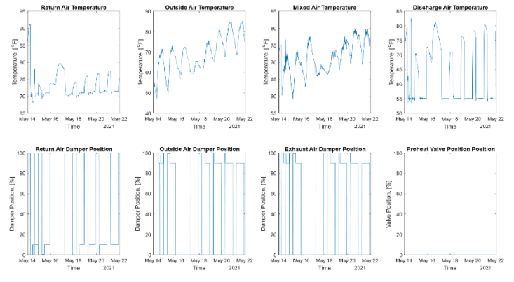
Fig. 4. BAS Data for AHU-2 and LE 100, 101, 105 for 05/14/2021-05/22/2021
