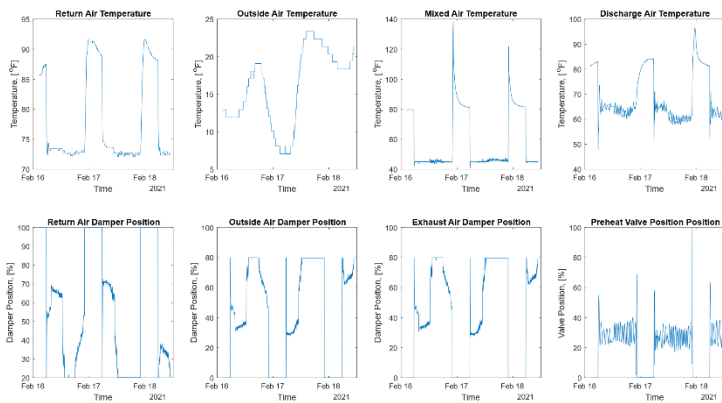
Fig. 3. BAS Data for AHU-2 and LE 100, 101, 105 for 02/16/2021-02/18/2021
